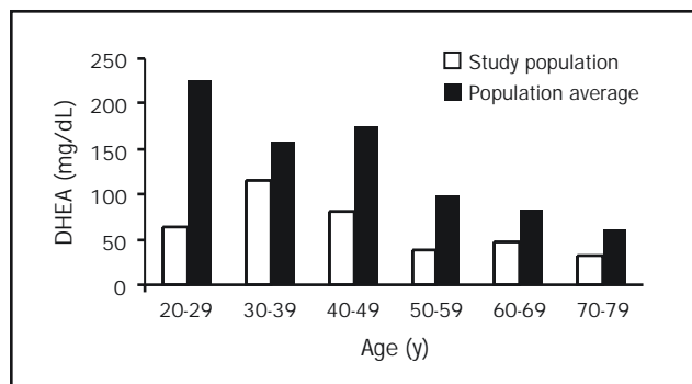
Figure 3. Dehydroepiandrosterone (DHEA) levels in women of all ages with reduced or absent libido compared with women with normal libido. P < .05 in all groups. Data from Guay and Jacobson. 89
