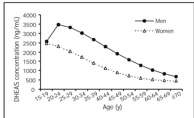
Figure 2. Changes in levels of circulating dehydroepiandrosterone sulfate (DHEAS) with aging. Reproduced from Orentreich et al 3 with permission from the Endocrine Society.
