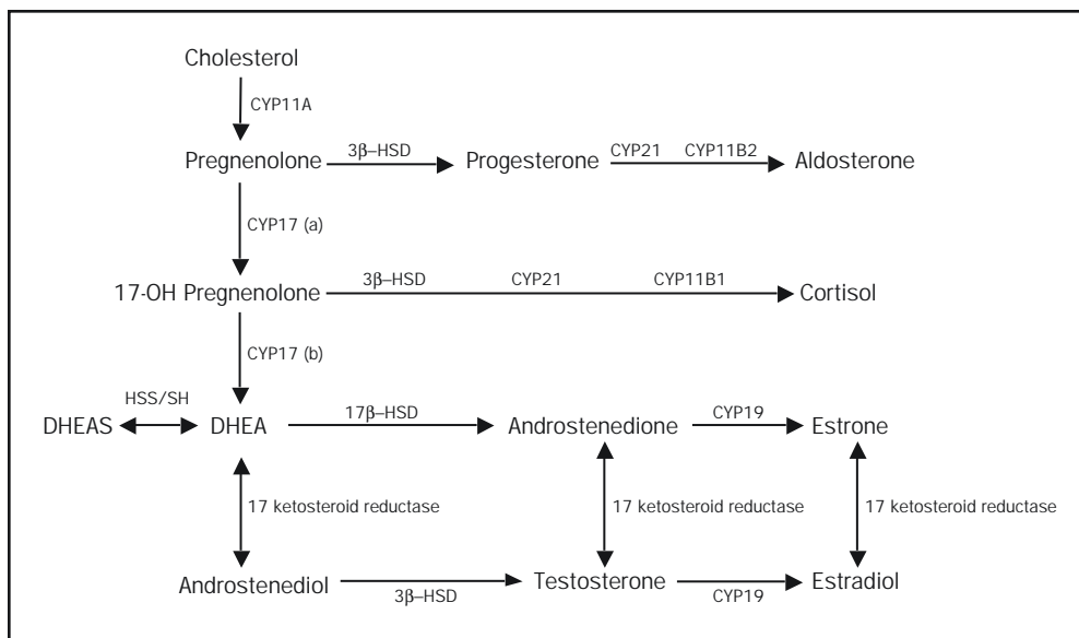
Figure 1. Simplified steroid synthesis pathway. CYP11A = 20,22 hydroxylase, 20,22-desmolase; CYP11B1 = 11β hydroxylase; CYP11B2 = 11β hydroxylase, 18-hydroxylase and 18-oxidase; CYP17 (a) = 17α hydroxylase (catalyzed by P-450 c17 ); CYP17 (b) = 17α-hydroxyprogesterone aldolase (catalyzed by P-450 c17 ); CYP19 = aromatase; CYP21 = 21 hydroxylase; DHEA = dehydroepiandrosterone; DHEAS = DHEA sulfate; 3β-HSD = 3β-hydroxysteroid dehydrogenase; 17β-HSD = 17β-hydroxysteroid dehydrogenase; HSS = 3β-hydroxysteroid sulfotransferase; SH = sulfohydrolase.
